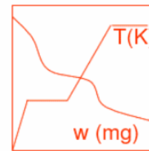
Quasi-Isotermo
